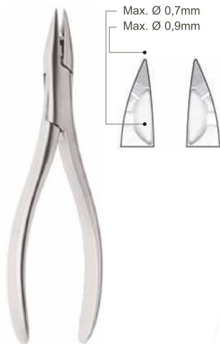
CDT-E-110 Universal Pliers for soft and hard wire 160mm
